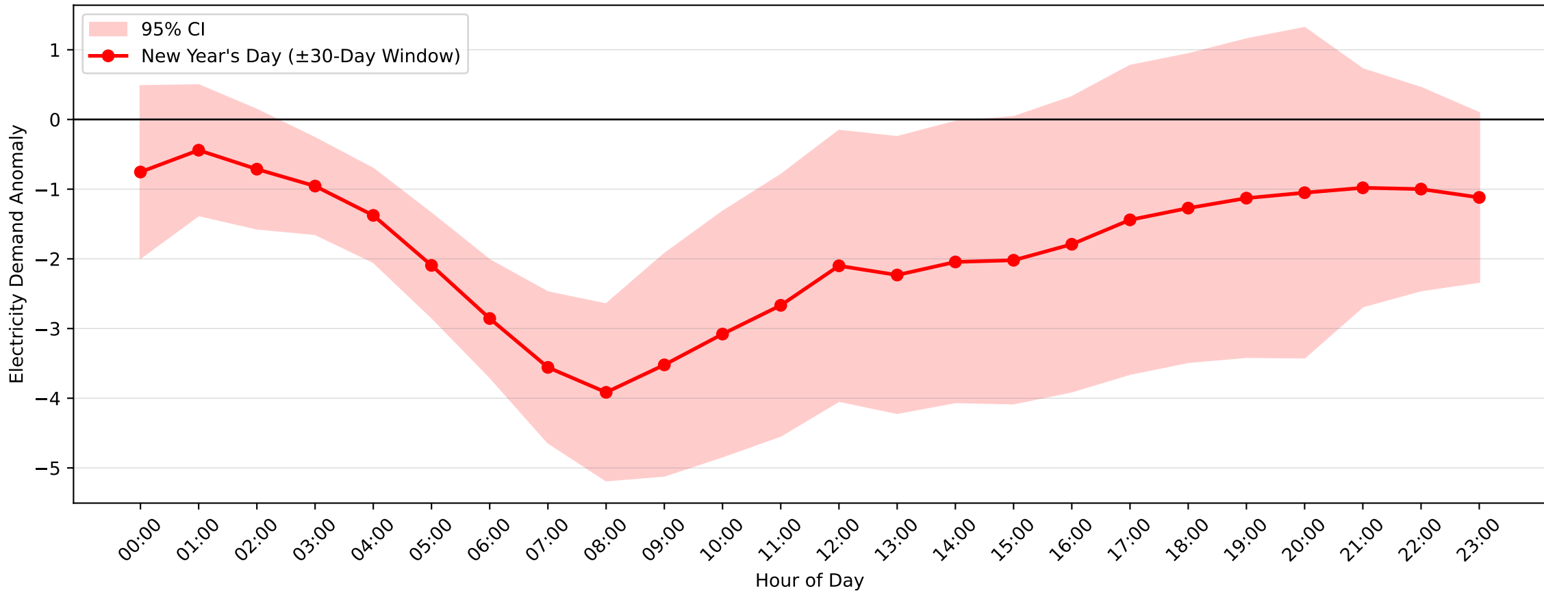
Bass Hill Demand Anomaly: New Year's Day (2004–2017, \pm 30 -Day Window)
